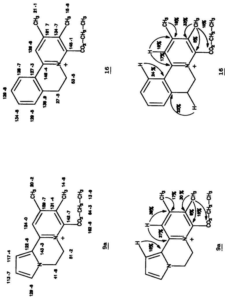
Fig 4. Assignment of ^{13}\text{C} -nmr chemical shifts of 9a and 16 and HETNOE measurements.
